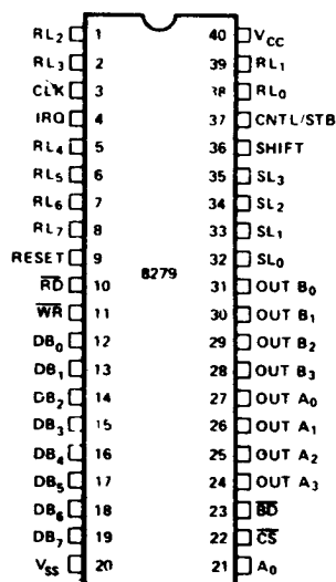
Figure 2. Pin Configuration
