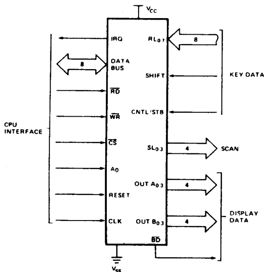
Figure 1. Logic Symbol
